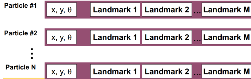
Figure 6.3 FastSLAM
